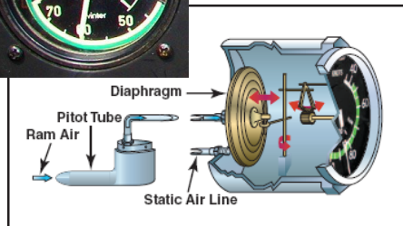
Calibrated Airspeed Indicator
