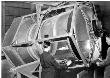
5-ft Free Flight Wind Tunnel
