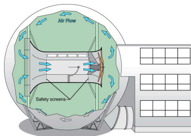
12-ft Free Flight Wind Tunnel
