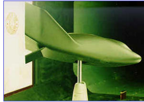
High-Angle-of-Attack Sting Balance
