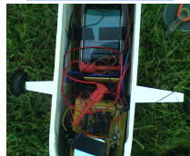
iPhone Installation
